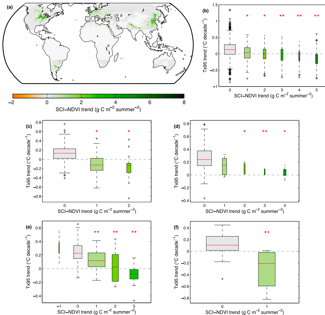
FIG. 16. (a) The SCI index calculated using GIMMS NDVI data instead of SIF to calculate the VEGsf (SCI-NDVI). Associations between SCI-NDVI and 95th-percentile summer temperature trends for (b) central North America, (c) northern North America, (d) northern East Asia, (e) southern East Asia, (f) and southern South America.
