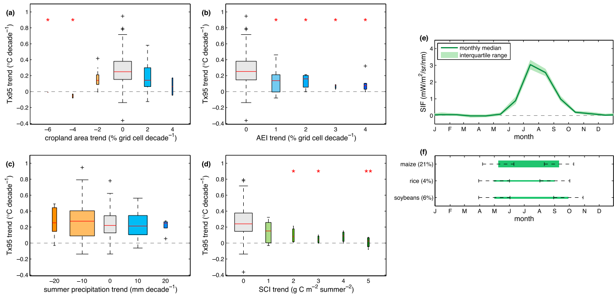
FIG. 11. As in Figs. 6 and 7, but for northern East Asia. Phenology is shown in (e) and (f) for the major crop production areas of northeastern China.
