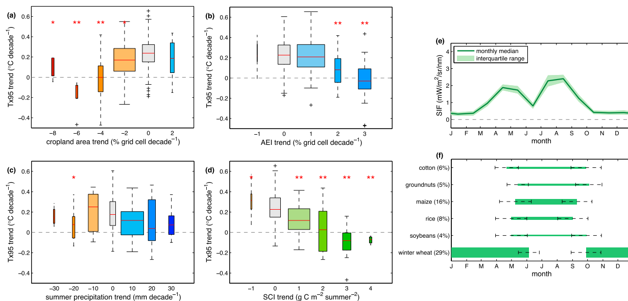
FIG. 12. As in Figs. 6 and 7, but for southern East Asia. Phenology is shown in (e) and (f) for the major crop production areas of the North China Plain.
