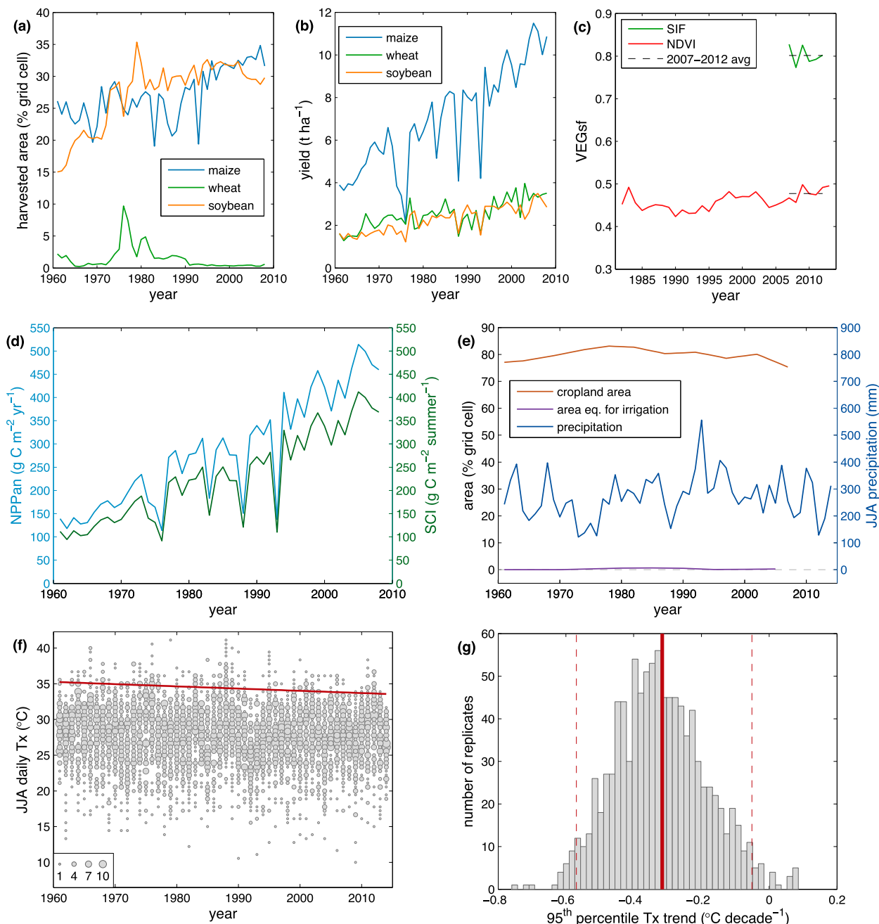
FIG. 5. An example showing local crop and land-use characteristics, weather data, and 95th-percentile maximum temperature trends for a weather station in Redwood County, Minnesota. (a) Crop harvested areas and (b) crop yields for all crops (of the six considered) where the maximum harvested area was greater than 1% of gridcell area. (c) The VEGsf as calculated using SIF and NDVI. (d) NPPan and SCI, calculated using crop harvested area, crop yield, and SIF-based VEGsf according to Eqs. (1)–(4). (e) Cropland area, area equipped for irrigation, and summer (JJA) precipitation are also considered as predictors of changing extreme temperatures. (f) Daily summer maximum temperature observations, with the 95th-percentile quantile regression trend overlaid in maroon. The quantile regression trend is calculated after adding jitter to the observations to account for rounding artifacts. (g) A histogram of 95th-percentile maximum temperature trends derived from a block-bootstrap resampling of yearly observations. The trend line fit using all the data is shown in the thick maroon line, and dashed lines indicate the 95% confidence interval on the trend. All land-use data are extracted for the nearest grid cell to the weather station, and gridded data are used at the original resolution of each dataset ( 5' for the crop harvested area and yield data, 5' for the irrigation data, and 1/2^{\circ} for the cropland area data).
