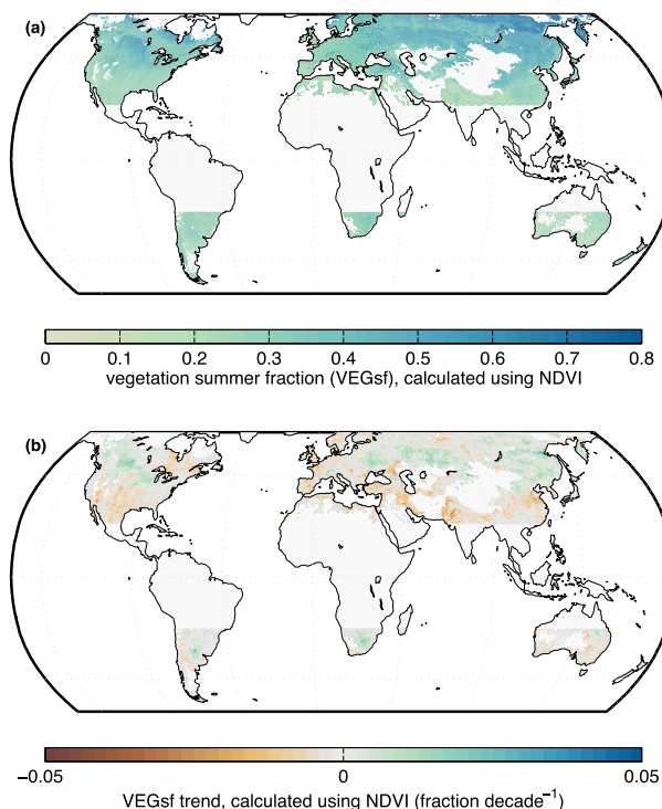
FIG. 15. (a) VEGsf calculated using the GIMMS NDVI data over 2007–12, consistent with the calculation for SIF. (b) The decadal trend in VEGsf calculated using GIMMS NDVI data over 1982–2013. Areas where VEGsf was not calculated using the SIF data are masked.
