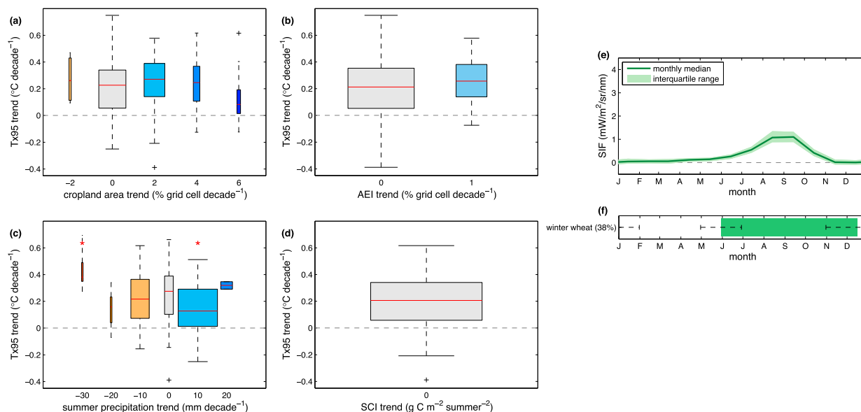
FIG. 13. As in Figs. 6 and 7, but for southern Australia. Phenology is shown in (e) and (f) for the major crop production areas of Western Australia.
