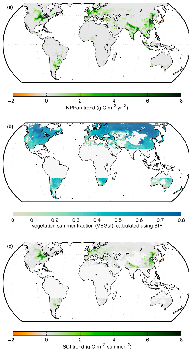
FIG. 3. (a) Trends in NPPan over 1961–2014, calculated using harvested area and yield records for six major crops: maize, wheat, rice, soybean, barley, and rapeseed. (b) The VEGsf, calculated using SIF from the GOME-2 satellite instrument. (c) Trends in the SCI index, calculated by multiplying NPPan trends and VEGsf.
