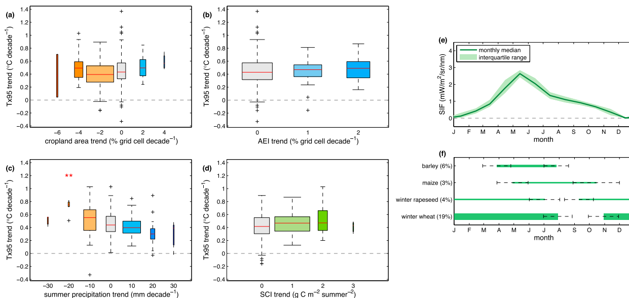
FIG. 10. As in Figs. 6 and 7, but for western Europe. Phenology is shown in (e) and (f) for the major crop production areas of southern England and northwestern France.
