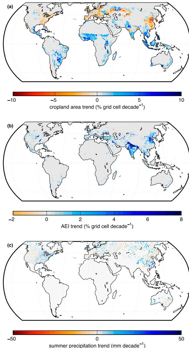
FIG. 2. (a) Trends in cropland area for 1961–2007, (b) trends in AEI for 1961–2005, and (c) trends in summer precipitation for 1961–2014. Cropland area is from a historical dataset based on satellite and agricultural census data (Ramankutty and Foley 1999). AEI is determined from agricultural census and land-use records as recorded by Siebert et al. (2015). Precipitation data are from the GHCND weather station dataset, and dot sizes are scaled according to Voronoi polygons surrounding each station. Summer seasons are defined as JJA in the Northern Hemisphere and DJF in the Southern Hemisphere.
