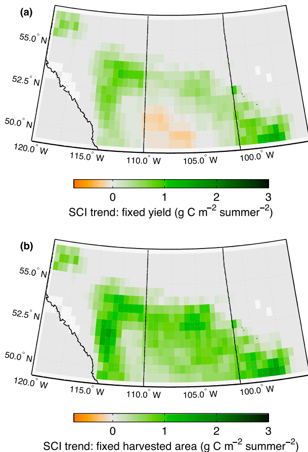
FIG. 9. Disaggregating contributions to SCI trends in the Canadian Prairies. (a) Trends in SCI calculated using yearly varying harvested area and average crop yields over 1961–2008. (b) Trends in SCI calculated using yearly varying yields and average harvested area. Note that the scale is truncated relative to Fig. 3 to better highlight differences between the calculations.
