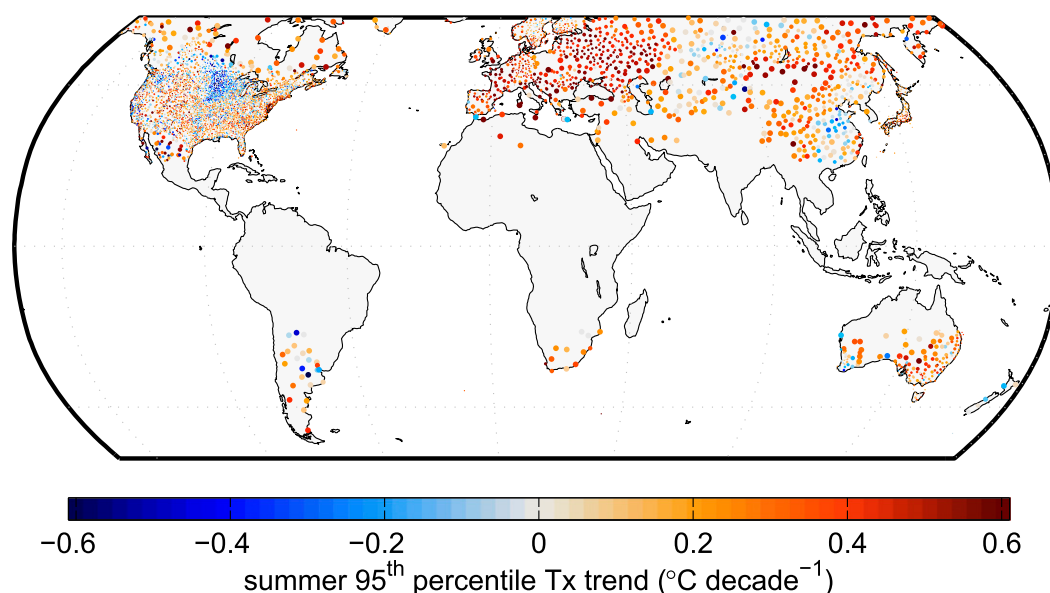
FIG. 4. Quantile regression trends in 95th-percentile summer daily maximum temperatures from 1961 to 2014. Temperature data are from the GHCND weather station dataset, and dot sizes are scaled according to Voronoi polygons surrounding each station. Summer seasons are defined as JJA in the Northern Hemisphere and DJF in the Southern Hemisphere.
