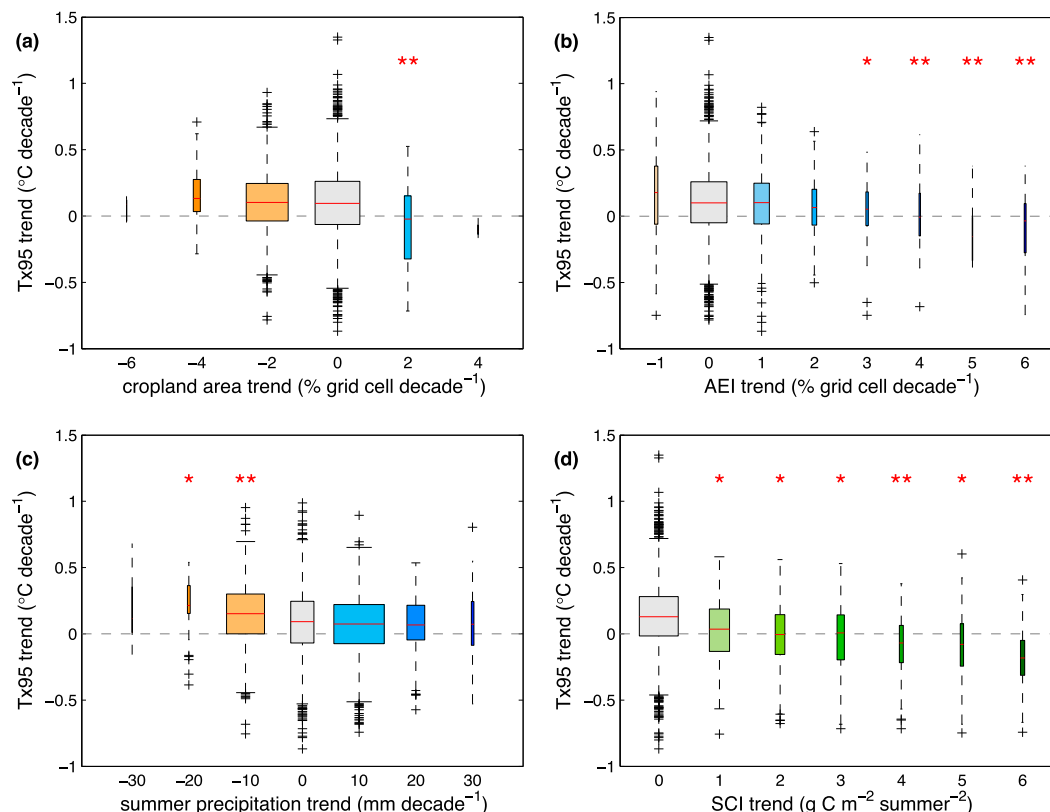
FIG. 6. Trends in central North American temperature extremes grouped according to candidate predictor variables: (a) cropland area, (b) AEI, (c) summer precipitation, and (d) SCI. Data points are from weather stations that have been associated with local (nearest \frac{1}{2}^\circ grid box) trends in land-use characteristics. Weather stations are evenly binned according to land-use or precipitation trends. Box-and-whisker plots display the full range of temperature trends across stations for each bin, with the boxes containing the interquartile range, whiskers extending up to 1.5 times the interquartile range, and crosses indicating outliers beyond this range. Asterisks indicate that 95th-percentile temperature trends for a given bin significantly differ from those in the control group (gray box, centered on zero trend) at the p < 0.05 level or p < 0.01 for double asterisks. The x -axis values are generally the midpoints of each bin, although edge bins include weather stations associated with outlier trends in each explanatory variable. Box widths are proportional to the area associated with the constituent weather stations except for the control bins that are narrowed by a factor of 5 for legibility. Box colors are consistent with the maps in Figs. 2 and 3.
