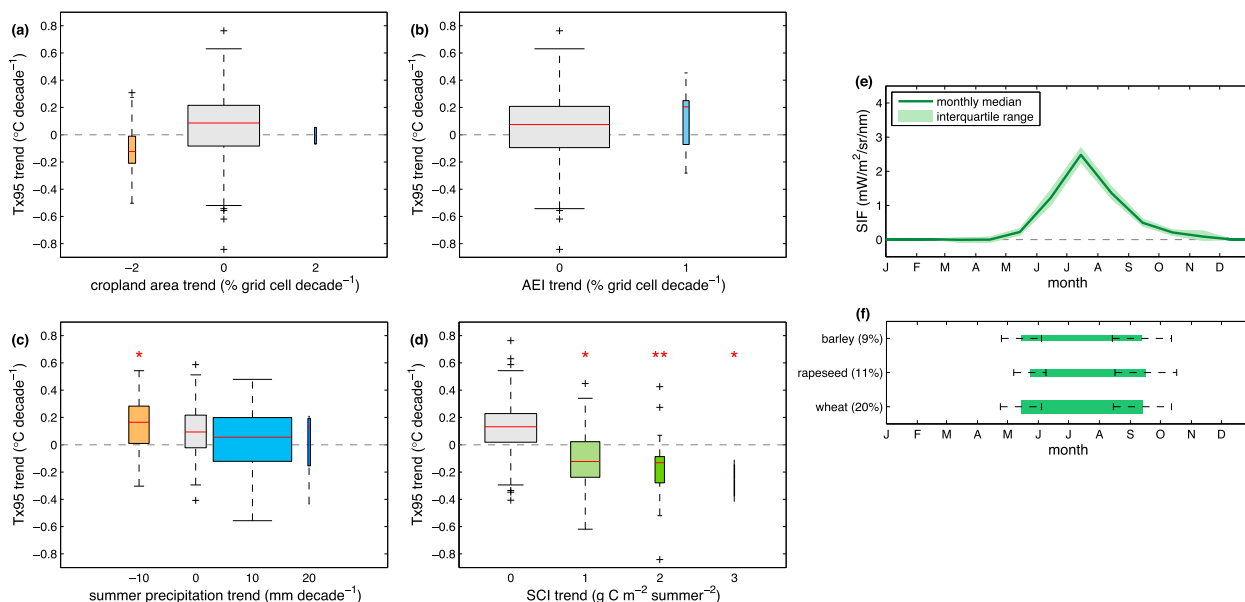
FIG. 8. As in Figs. 6 and 7, but for northern North America. One outlier station where the 95th-percentile summer temperature trend was >2^{\circ}\text{C decade}^{-1} has been removed from the box-and-whisker plots and statistical analysis. Phenology is shown in (e) and (f) for the major crop production areas of the Canadian Prairies.
