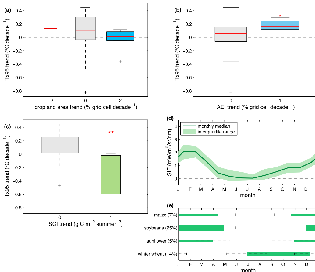
FIG. 14. As in Figs. 6 and 7, but for southern South America. Phenology is shown in (d) and (e) for the major crop production areas of the Argentine Pampas.
